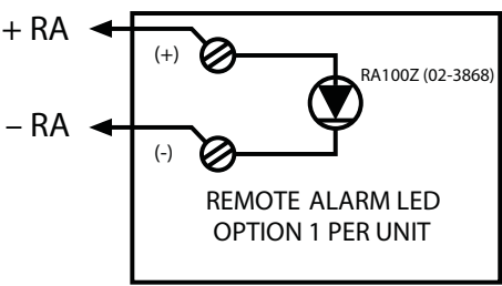
Wiring Diagram from 63-1158 to 02-3868
